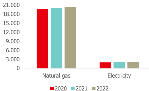
Energy efficiency (GJ/10 kton produced)
