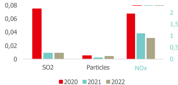
Atmospheric emissions (ton/10 kton produced)
